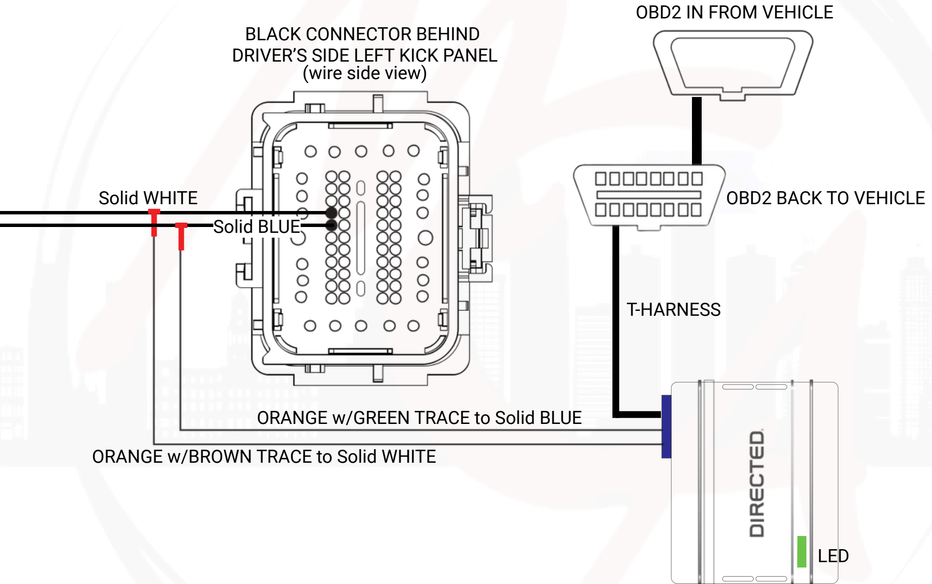
F18-SK REMOTE START INSTALLATION ILLUSTRATION
